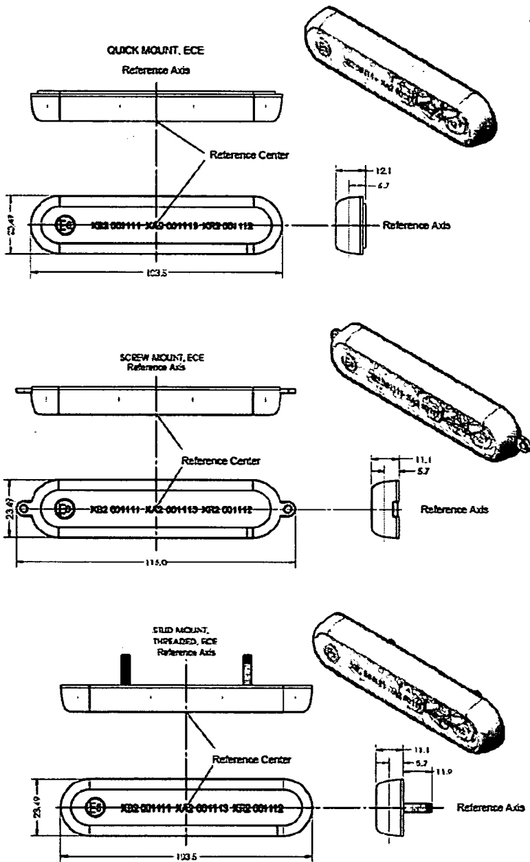
Optical Axis Drawing Location and Direction of Optical Axis
